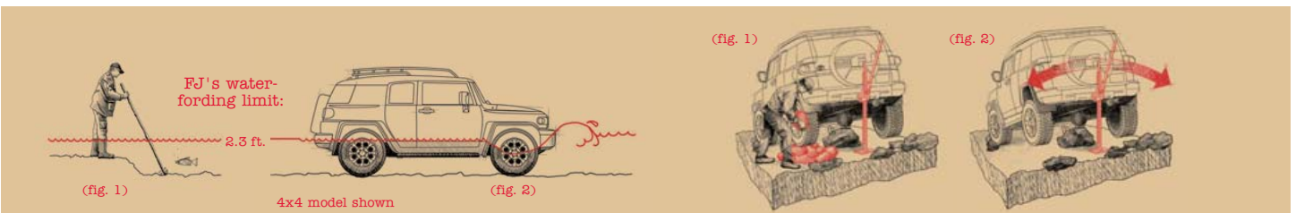
Fig. 1: When making a water crossing, walk the route first to determine depth, bottom firmness and obstacle location. Know the vehicle's water-fording 1 limit so the engine intake doesn't suck in water. Fig. 2: With your available transfer case in Low, cross slowly, but with enough speed to create a small bow wave, which can help protect engine components.
