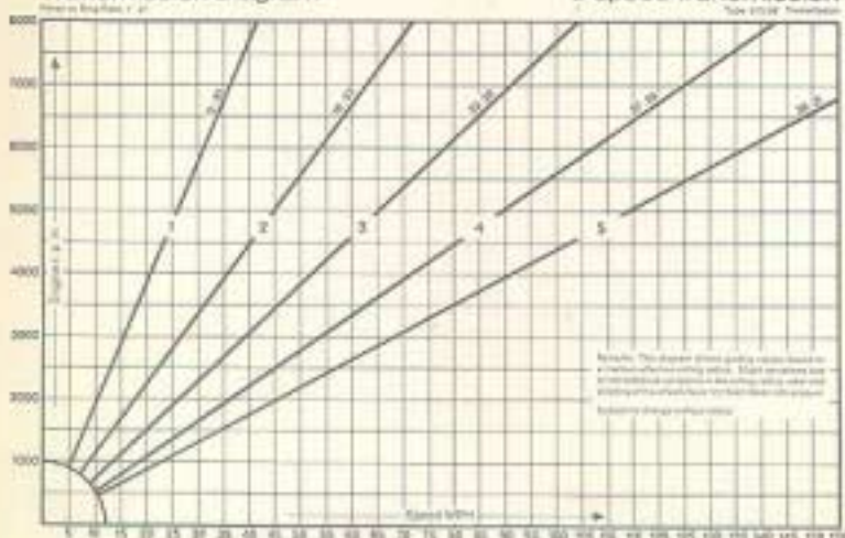
Transmission Diagram
